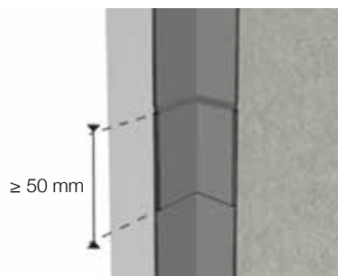
Figure 16 : Raccordement vertical
